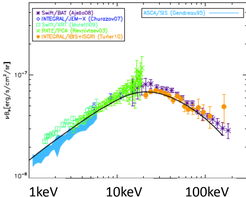
X-ray Background Spectrum
