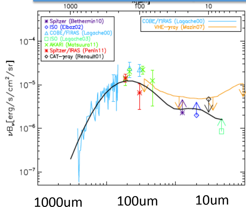
Infrared Background Spectrum
